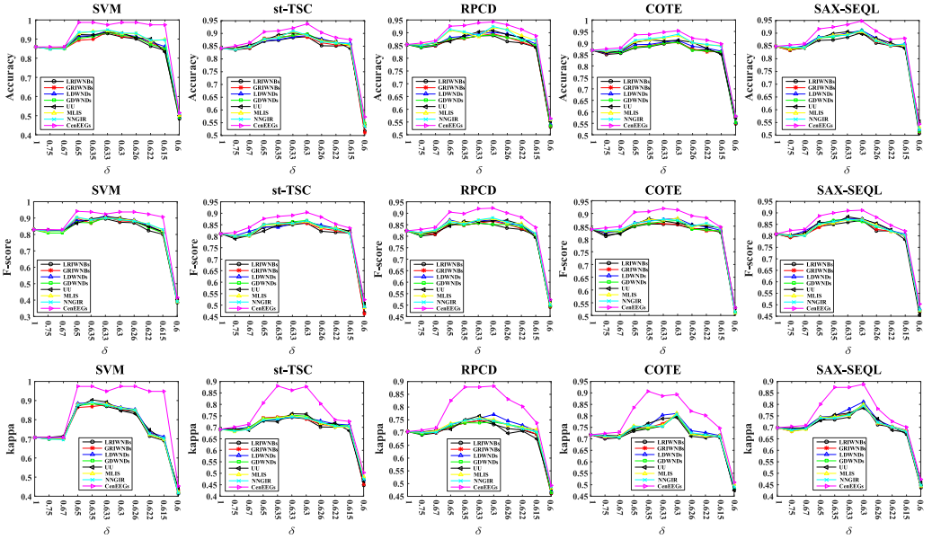
Fig. 5. Classification with different classifiers on EEG dataset #3.
