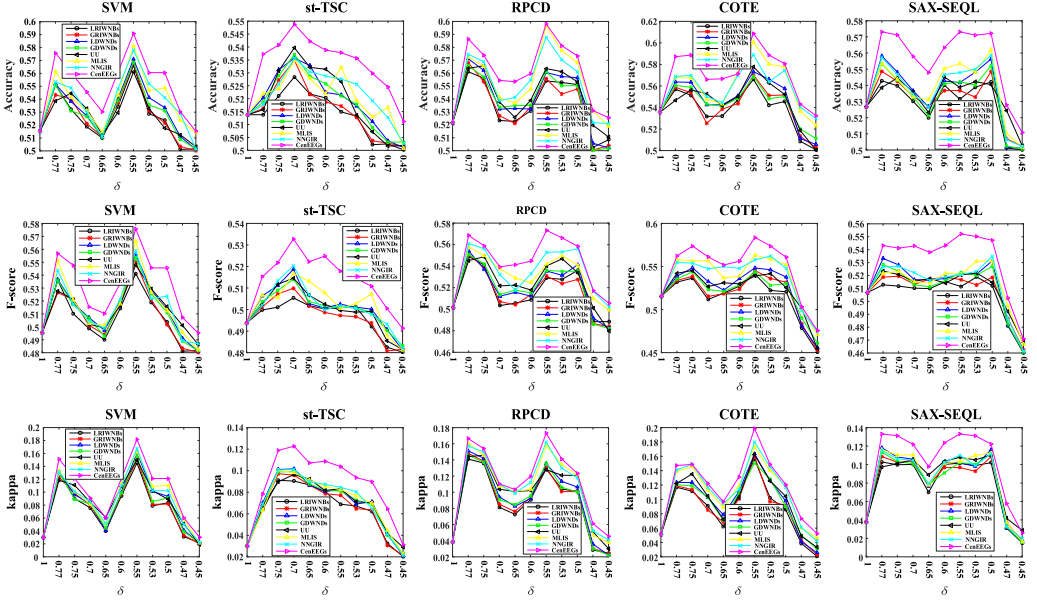
Fig. 4. Classification with different classifiers on EEG dataset #2.
