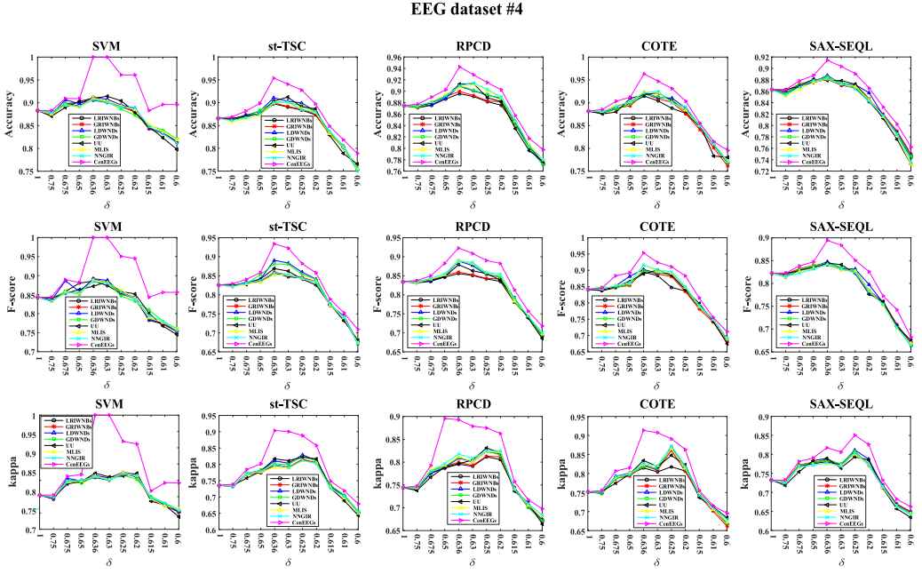
Fig. 6. Classification with different classifiers on EEG dataset #4.
