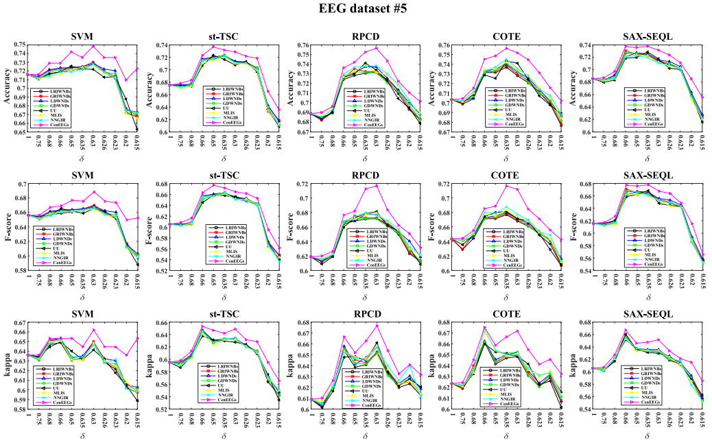
Fig. 7. Classification with different classifiers on EEG dataset #5.
