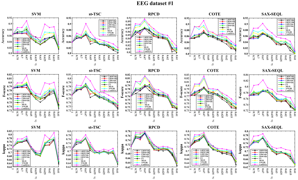
Fig. 3. Classification with different classifiers on EEG dataset #1.
